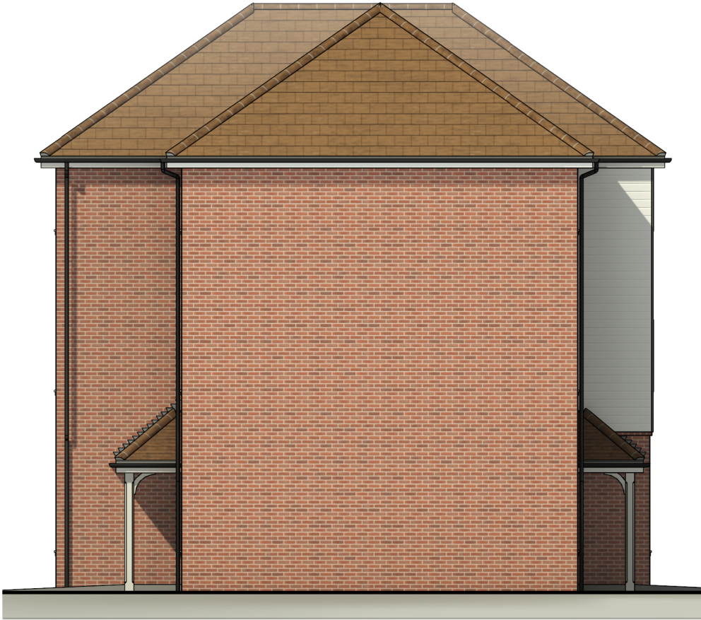
Left Elevation
