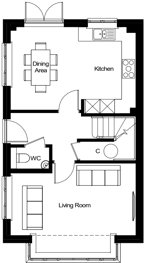
Ground Floor P033 - 4H2b
