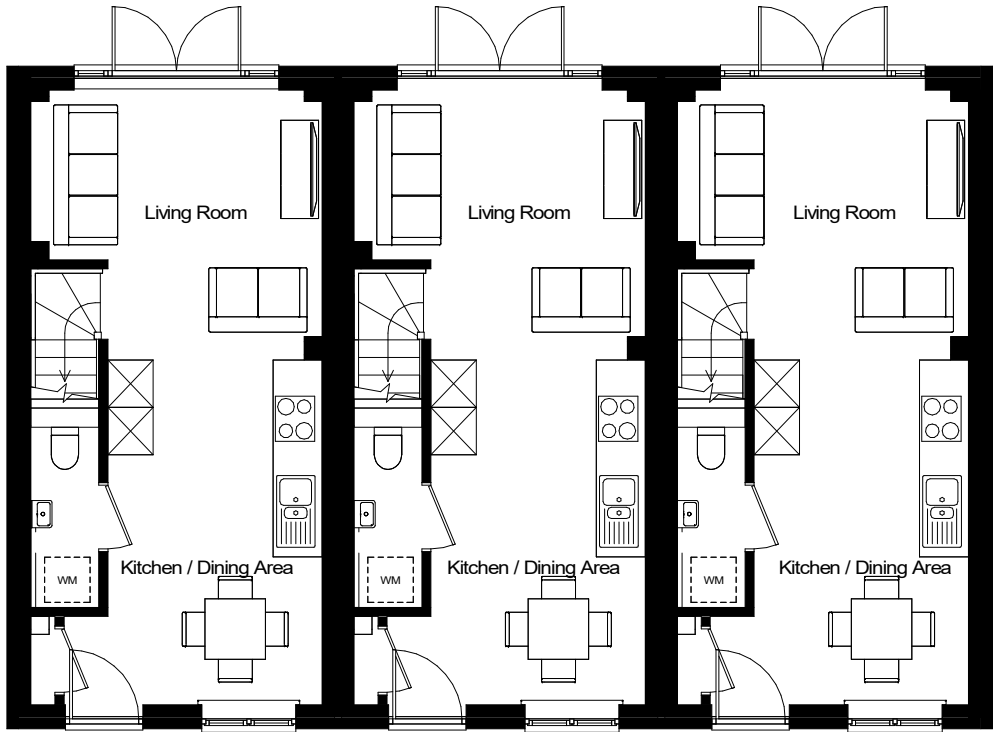
Ground Floor P036 - 2H2
