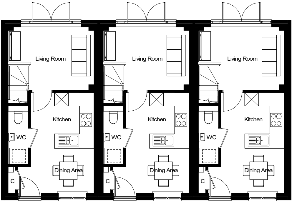
Ground Floor P039 - 2H1
