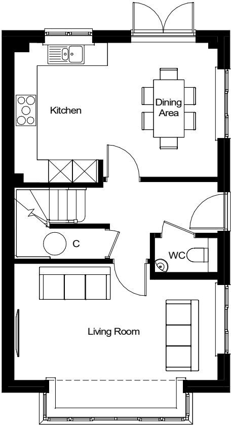
Ground Floor P043 - 4H2b
