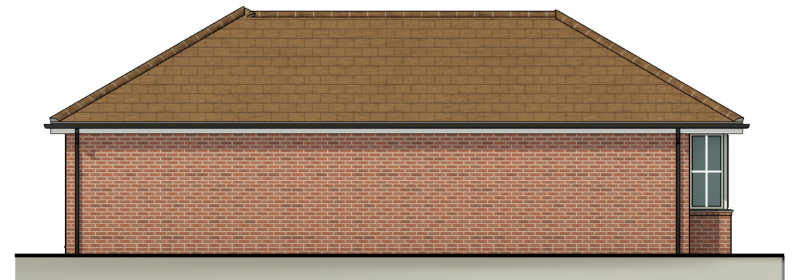
Left Elevation P045
