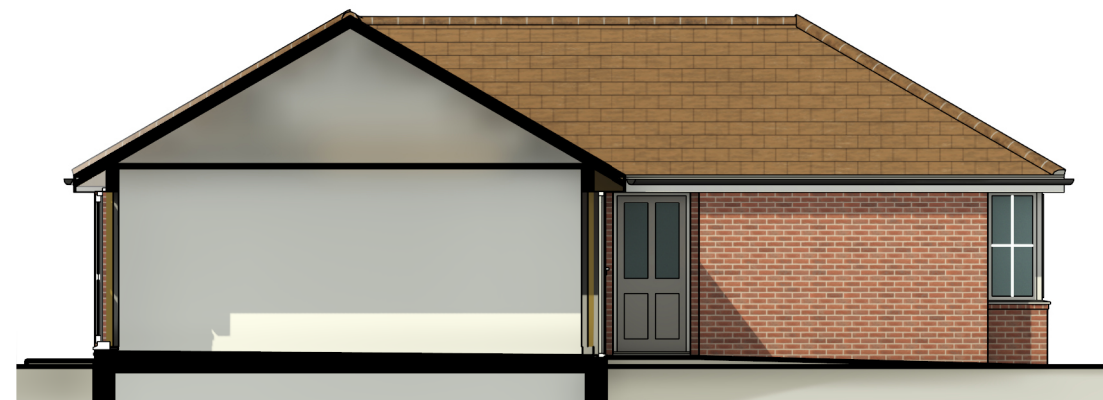
Right Elevation - Section P050
