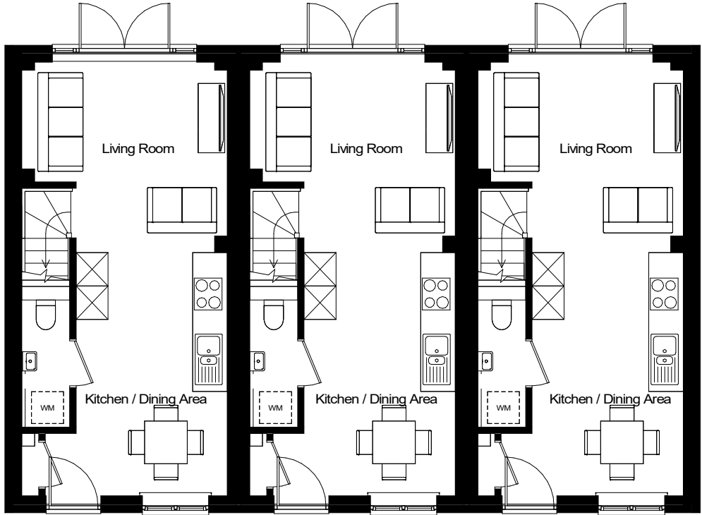
Ground Floor P053 - 2H2
