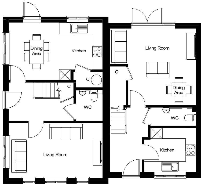
Ground Floor P064 - S3H2
