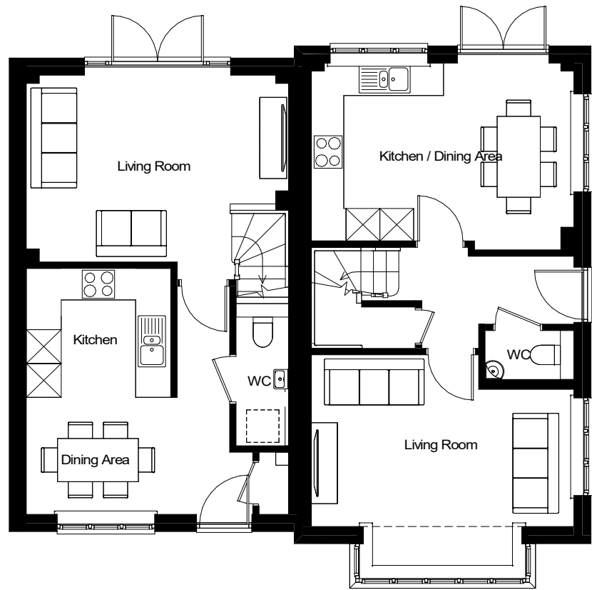
Ground Floor P066 - 3H2
