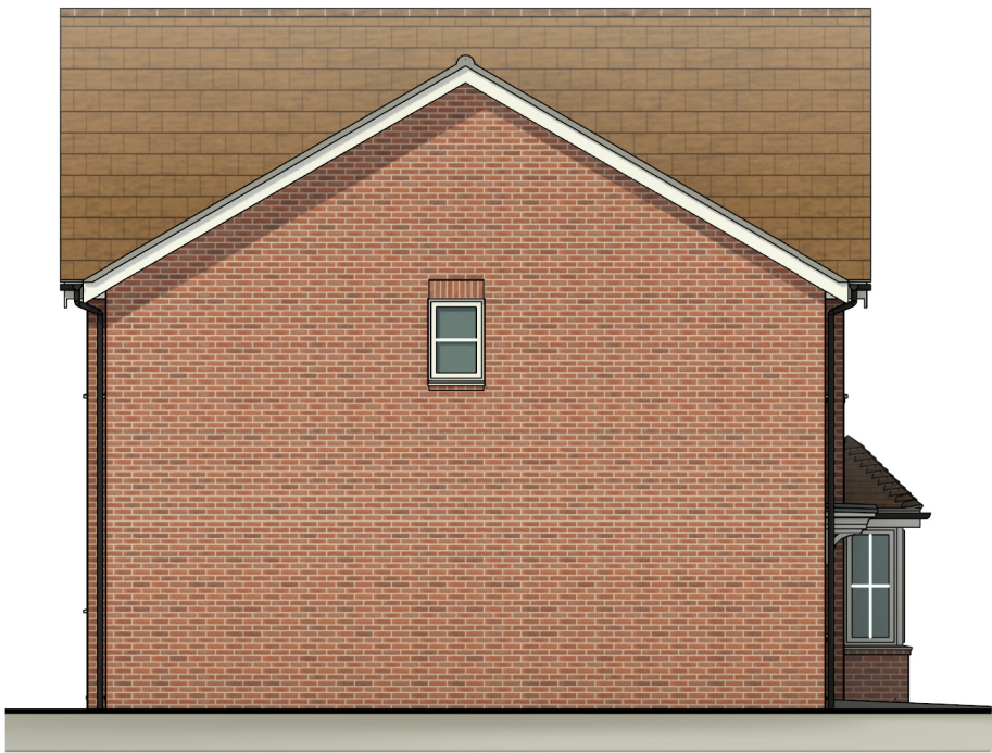
Left Elevation P066
