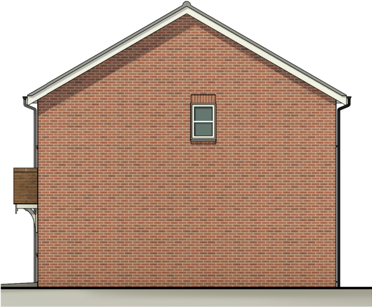
Right Elevation P069
