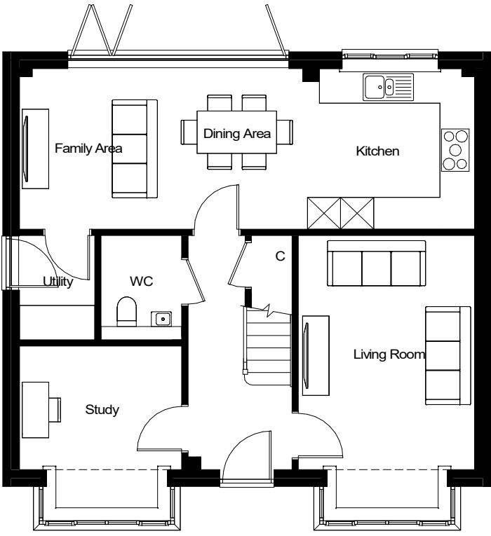
Ground Floor P071 - 4H4b
