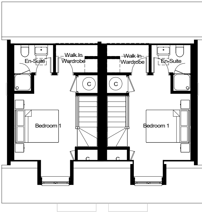
Second Floor
