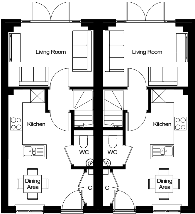
Ground Floor P074 - 3H5
