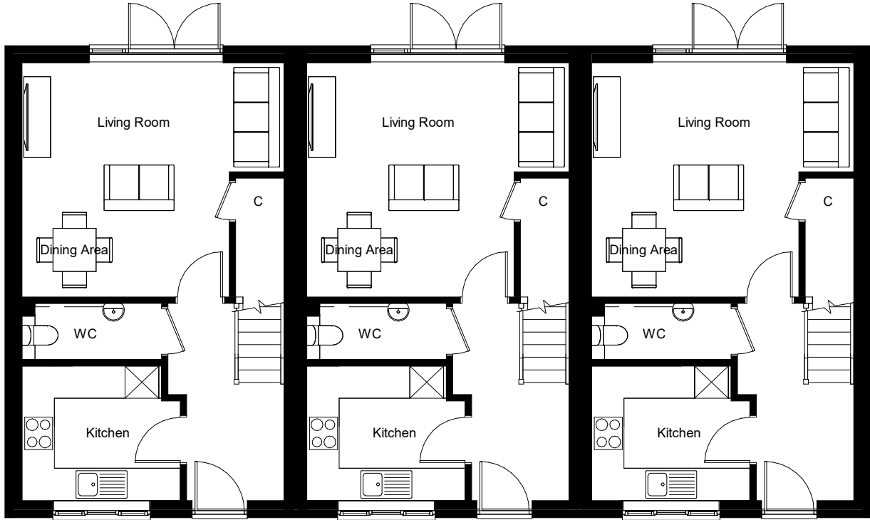
Ground Floor P079 - S2H1
