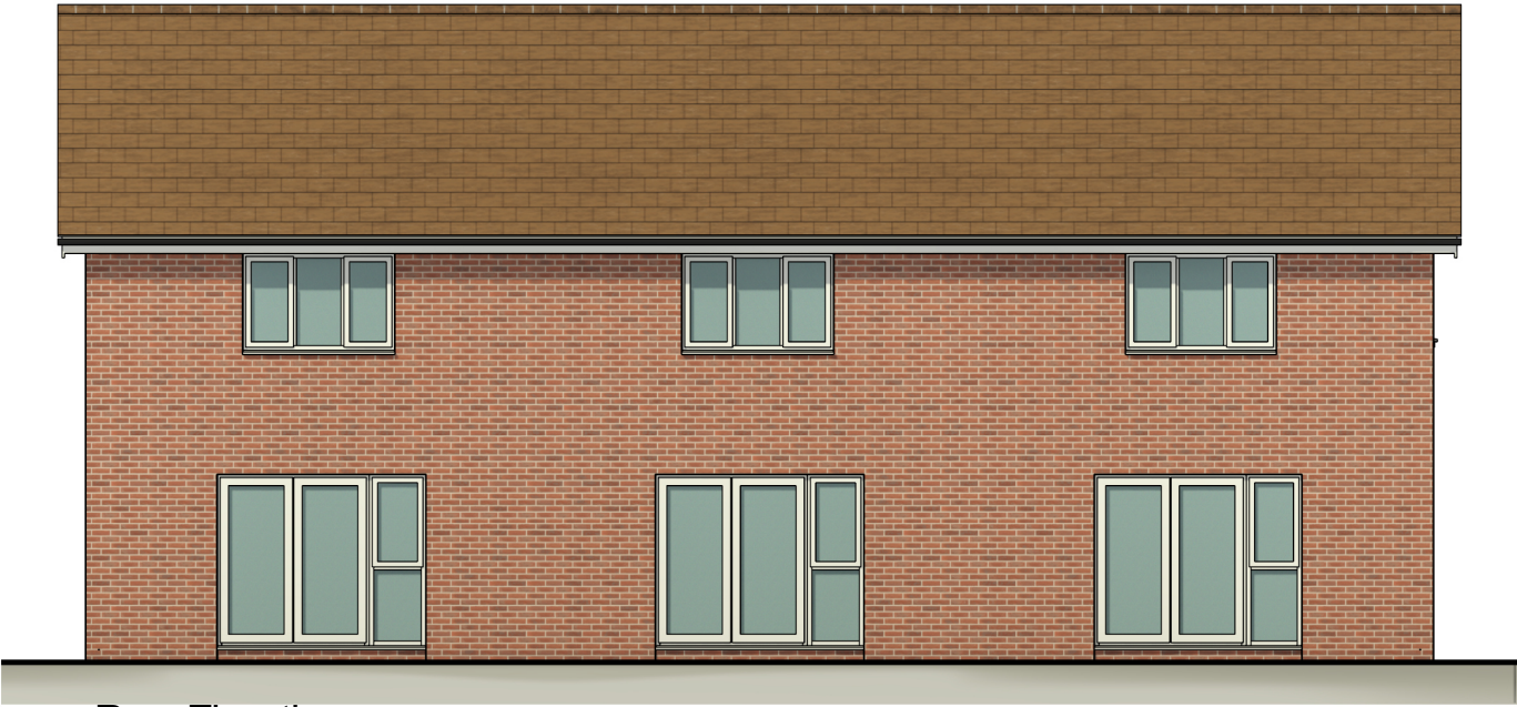
Rear Elevation P081
