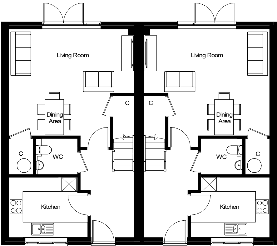
Ground Floor P082 - S3H1
