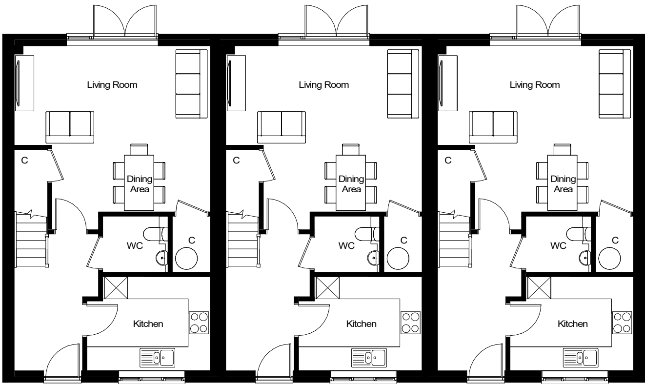
Ground Floor P090 - S3H1
