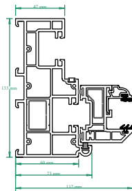
Top Sash
