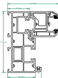
Top Sash
