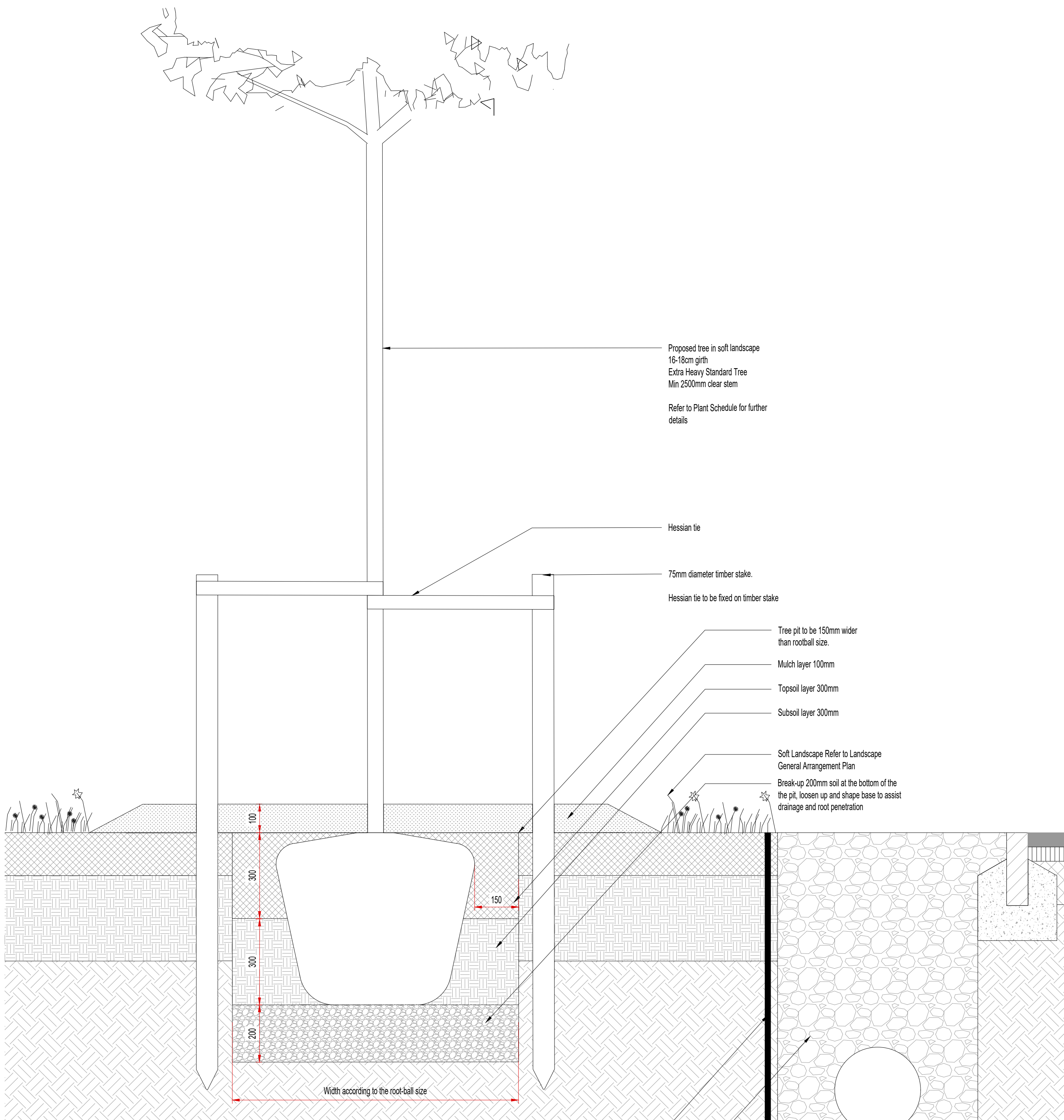
02 Tree in Soft Landscape Adjacent to Filter Drain - Typical Detail 745001 1:10
