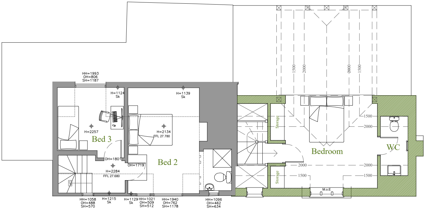
First Floor 1:100 | PROPOSED
