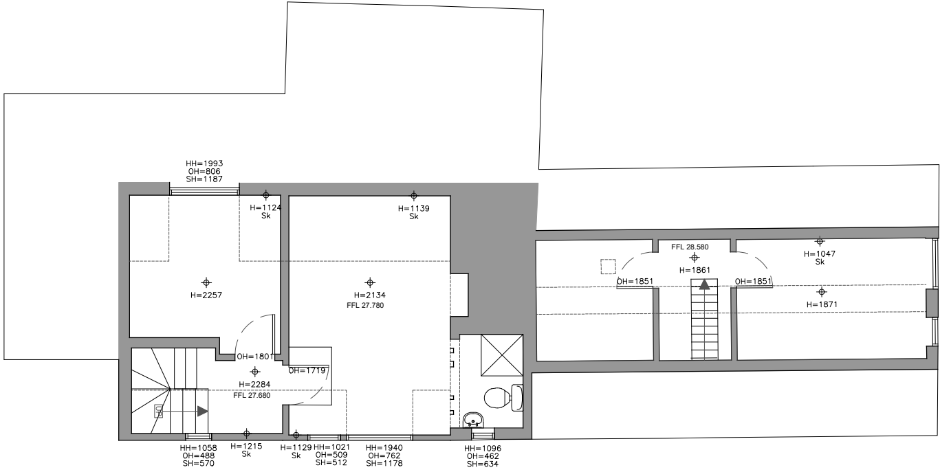
First Floor 1:100 | EXISTING
