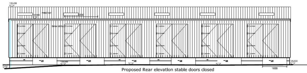
Proposed Rear elevation stable doors closed
