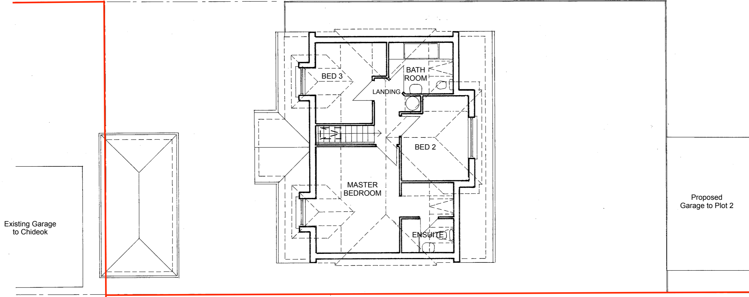
PROPOSED FIRST FLOOR PLAN TO PLOT 1 HOUSE
