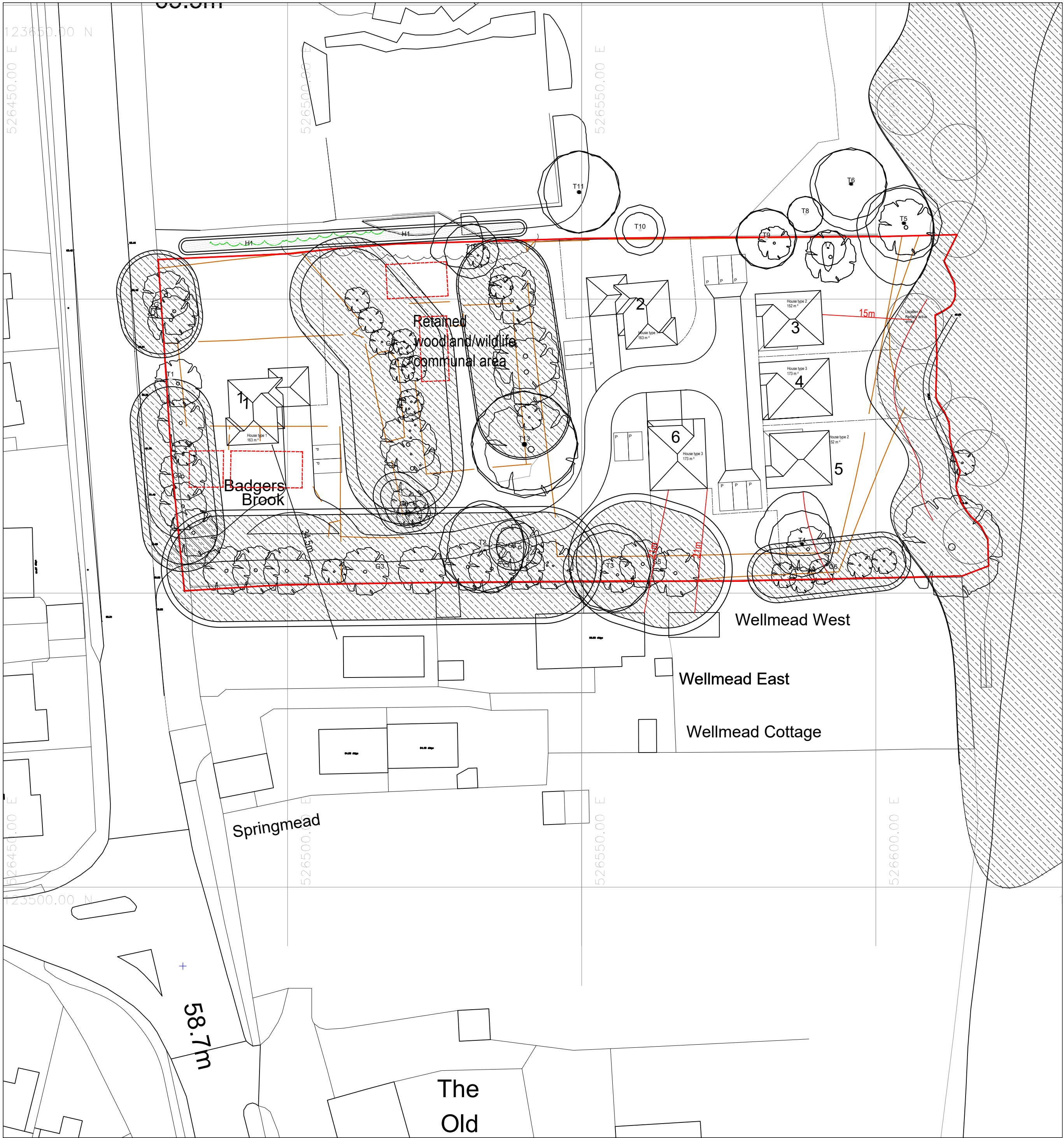
BLOCK PLAN
