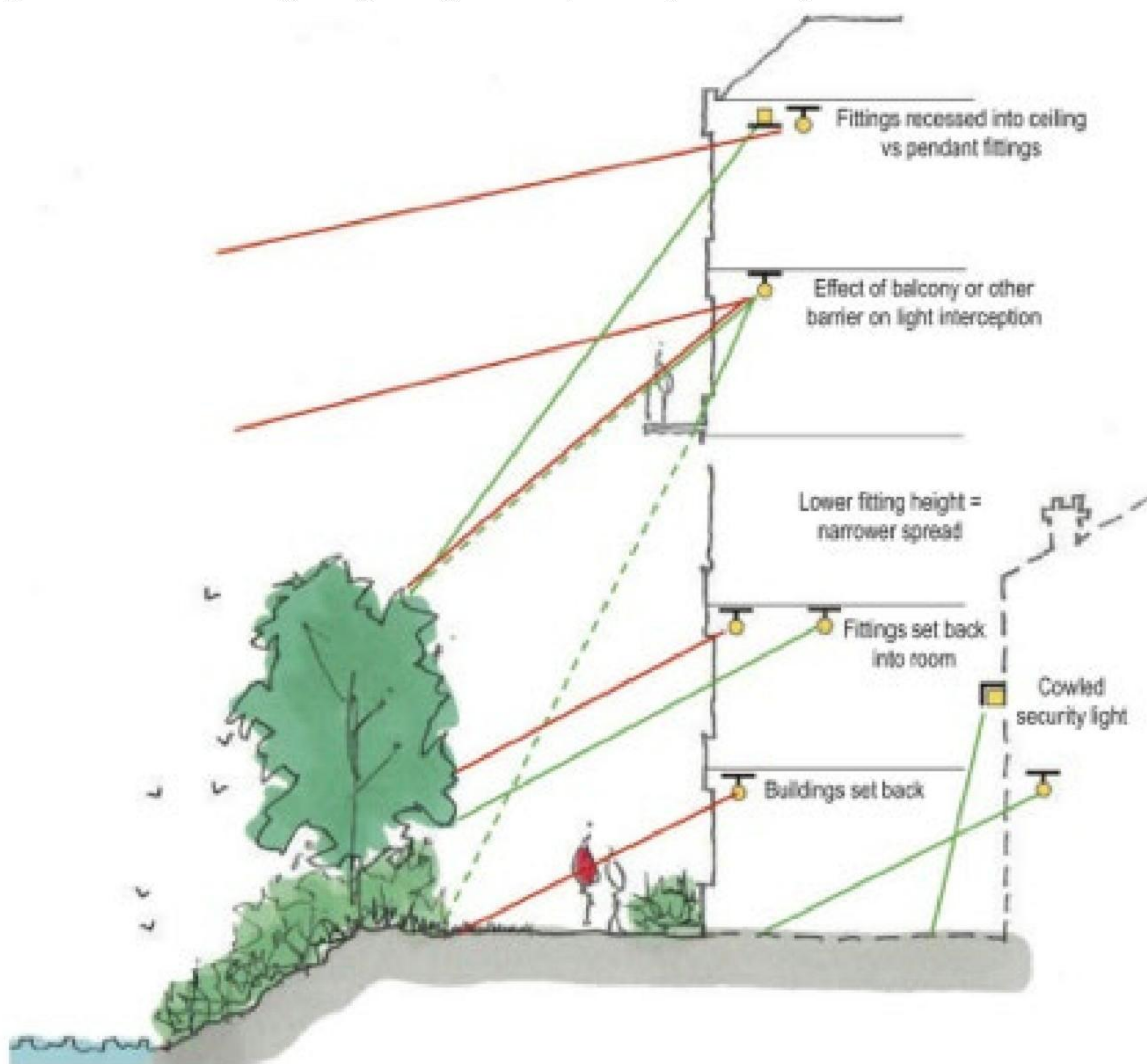
Figure 26. Internal lighting mitigation options (ILP 2023).
