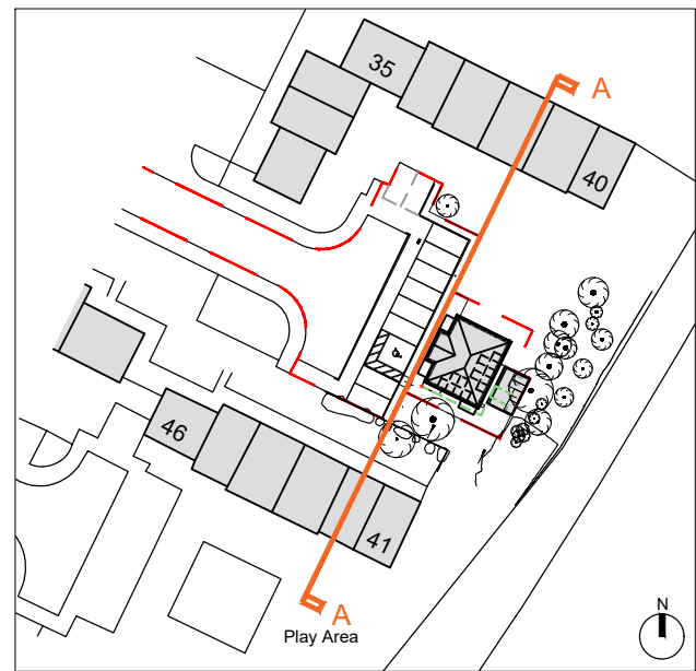
Street Scene Location Plan - Scale1:1000
