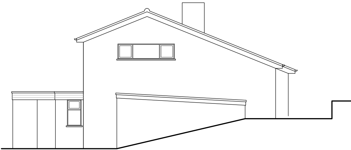
Existing RHS Elevation Scale 1/100@A3
