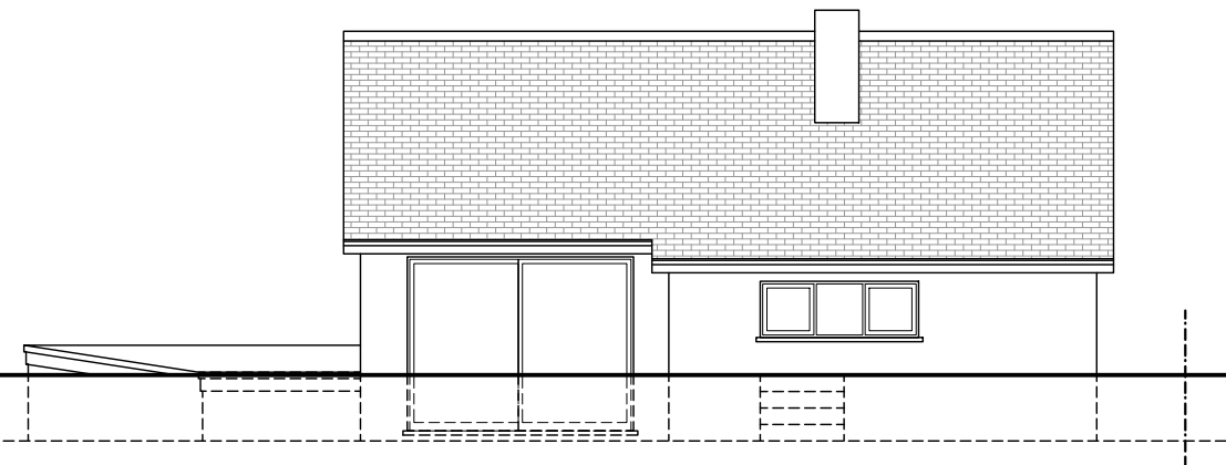
Existing Rear Elevation Scale 1/100@A3
