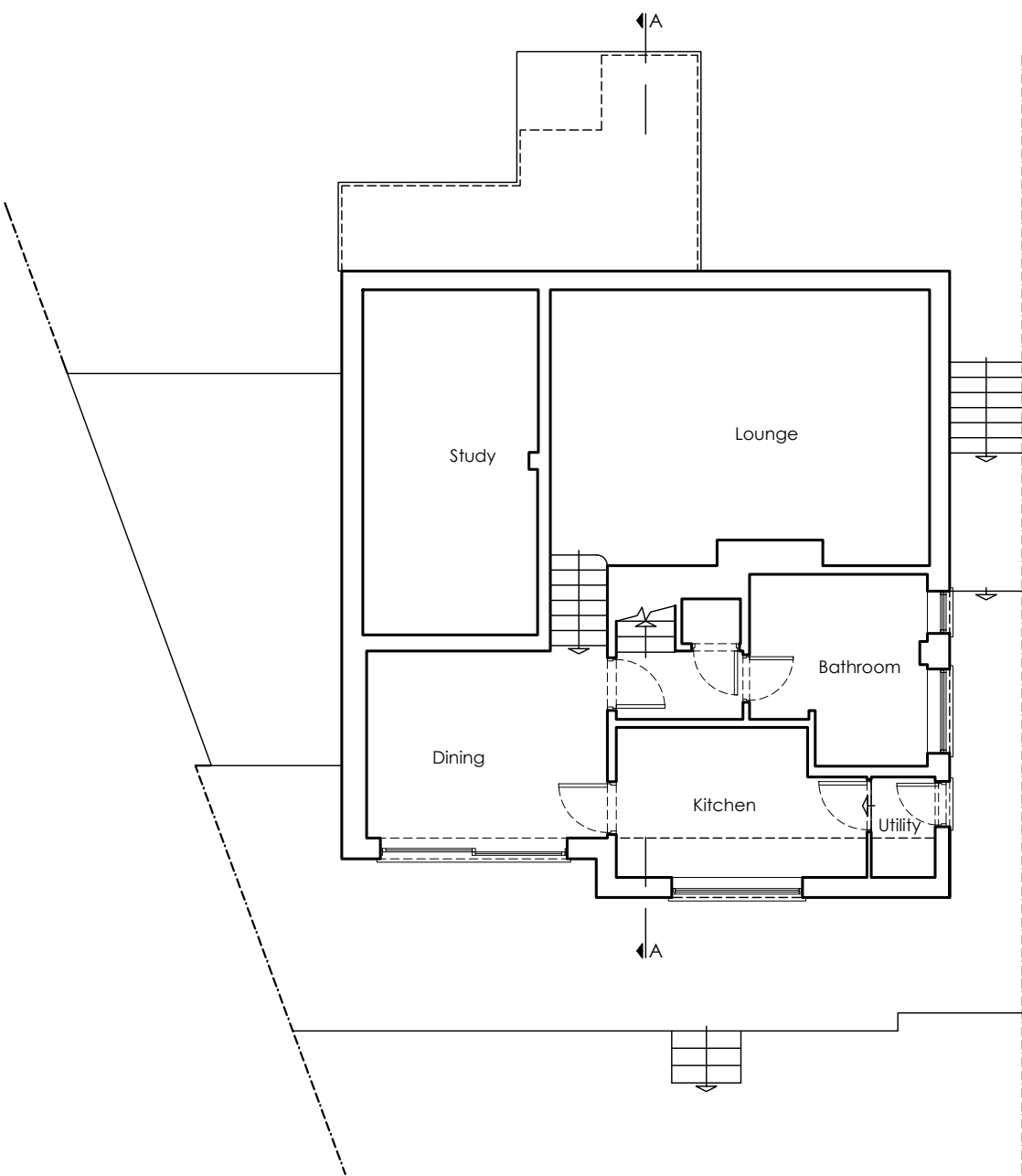
Existing Upper Ground Floor Plan Rear Garden Level Scale 1/100@A3
