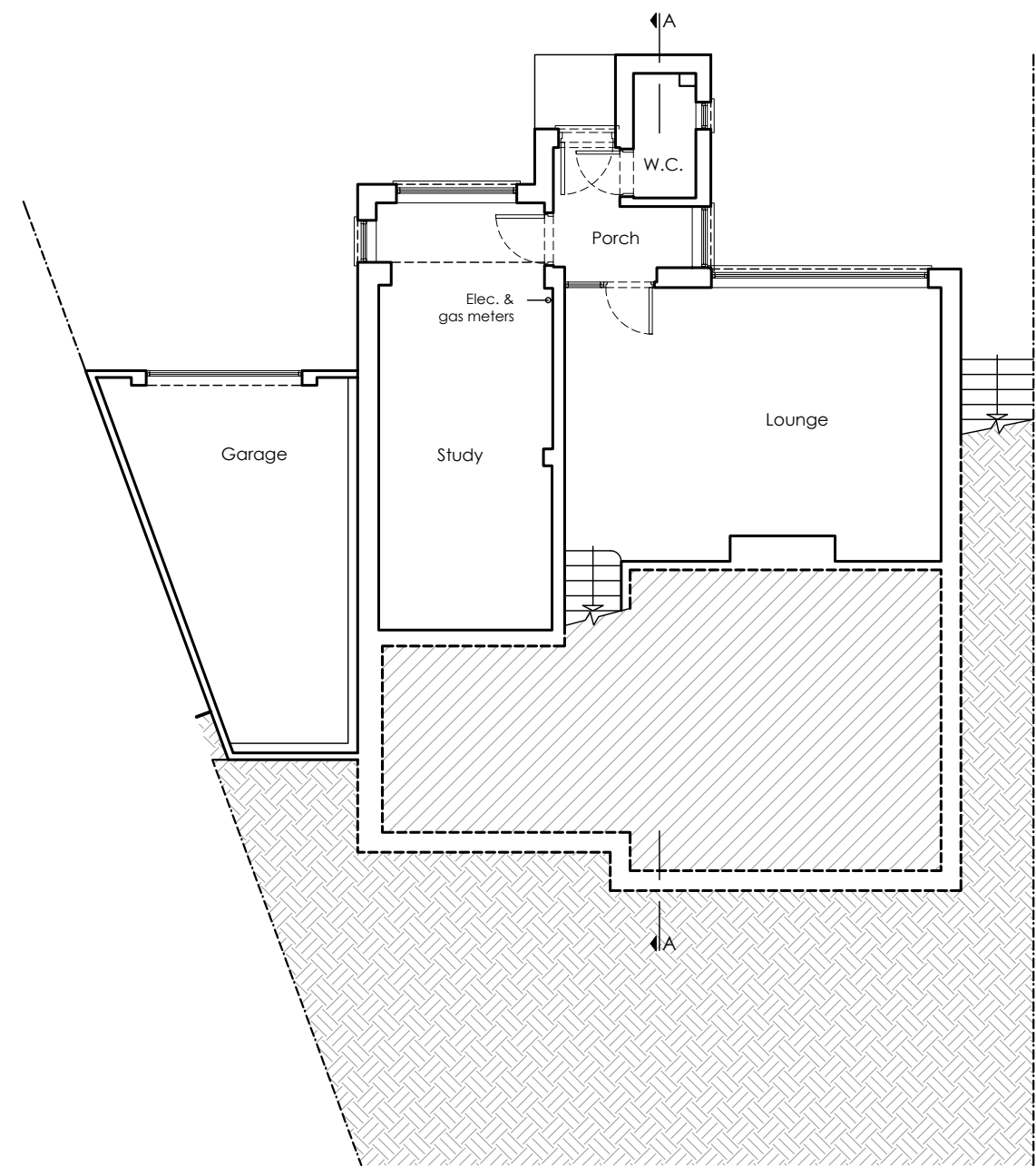
Existing Lower Ground Floor Plan Street Level Scale 1/100@A3
