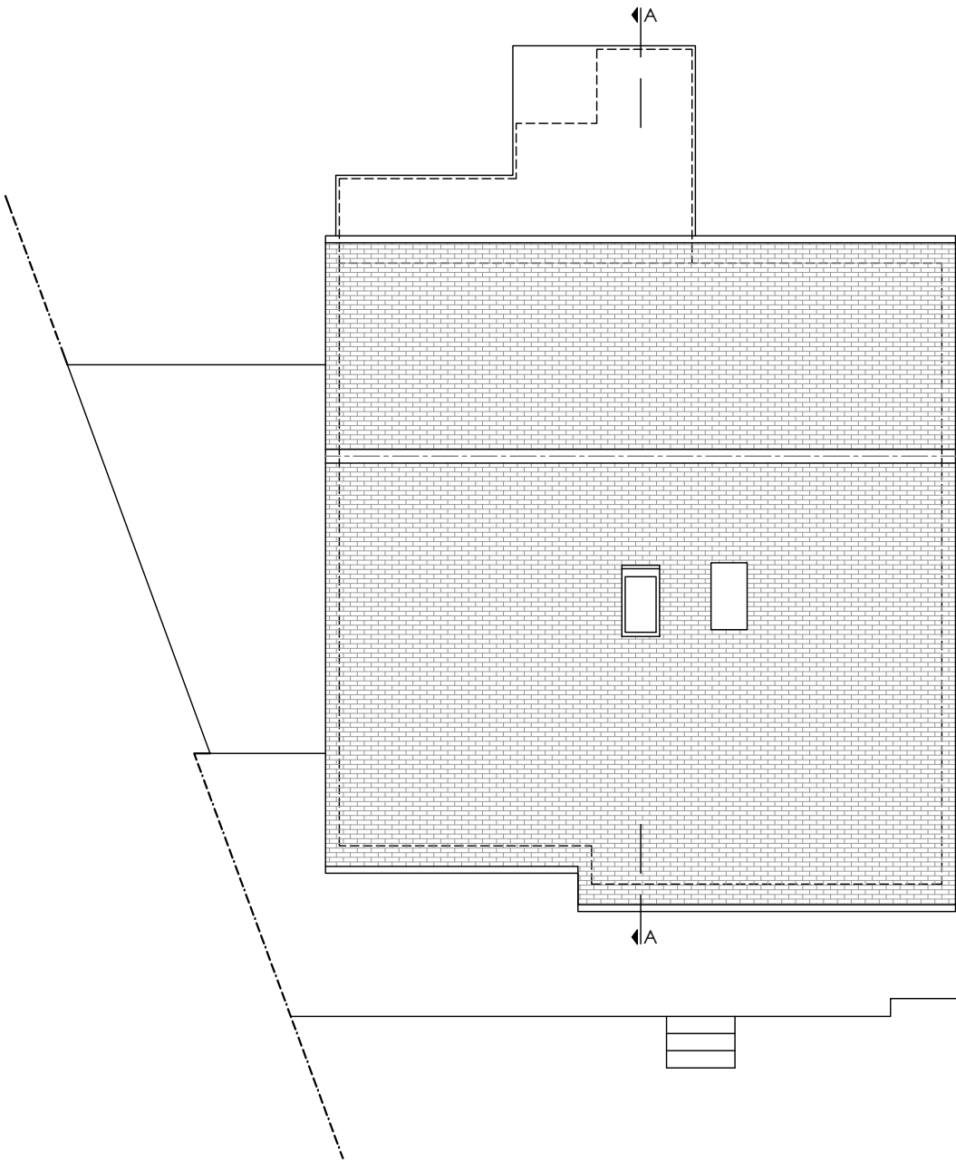
Existing Roof Plan Scale 1/100@A3
