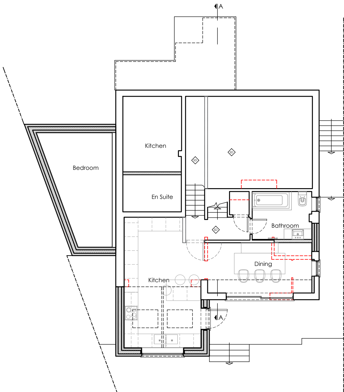
Proposed Upper Ground Floor Plan Rear Garden Level Option C Scale 1/100@A3
