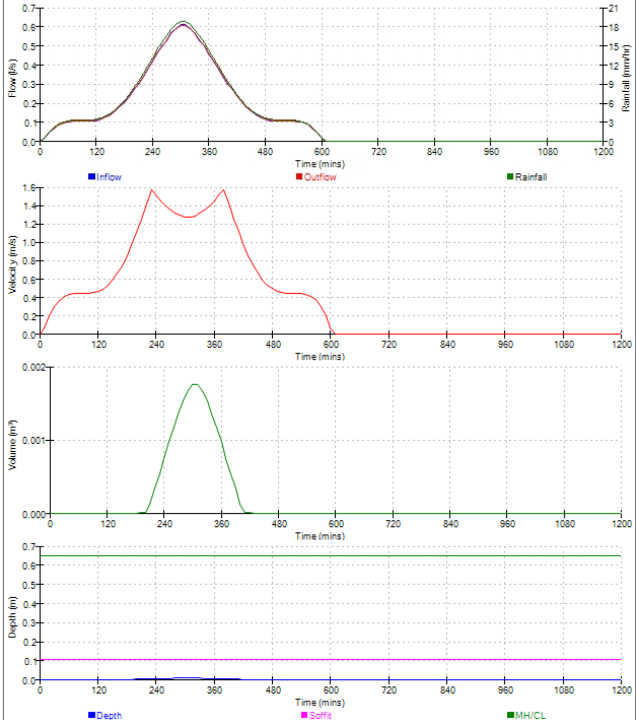
Graphs for Pipe 2.001 US/MH S2 (Storm) 600 minute 100 year winter Status: OK
