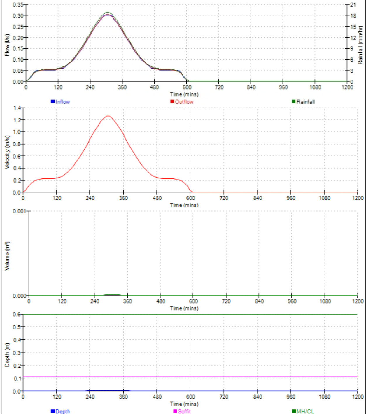
Graphs for Pipe 1.000 US/MH RE1 (Storm) 600 minute 100 year Winter Status: OK
