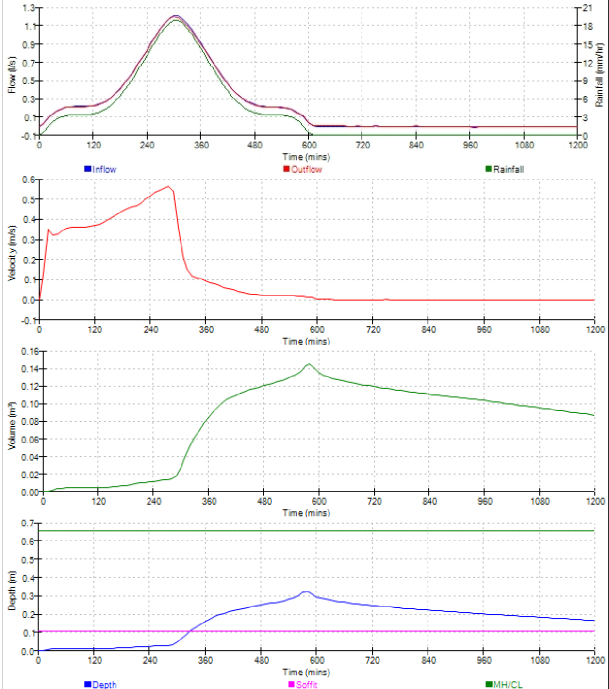
Graphs for Pipe 1.002 US/MH S3 (Storm) 600 minute 100 year winter Status: SURCHARGED
