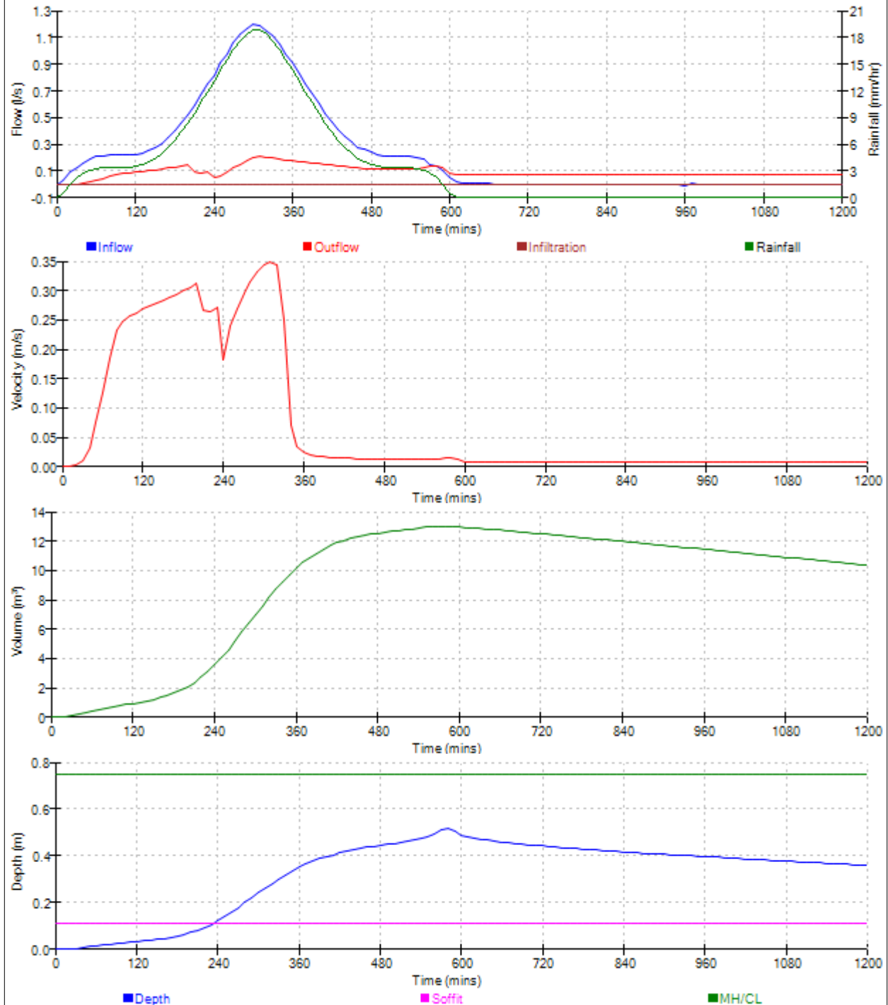
Graphs for Pipe 1.003 US/MH S4 (Storm) 600 minute 100 year winter Status: SURCHARGED
