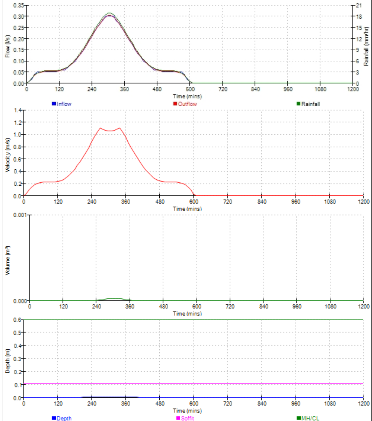
Graphs for Pipe 2.000 US/MH RE2 (Storm) 600 minute 100 year Winter Status: OK
