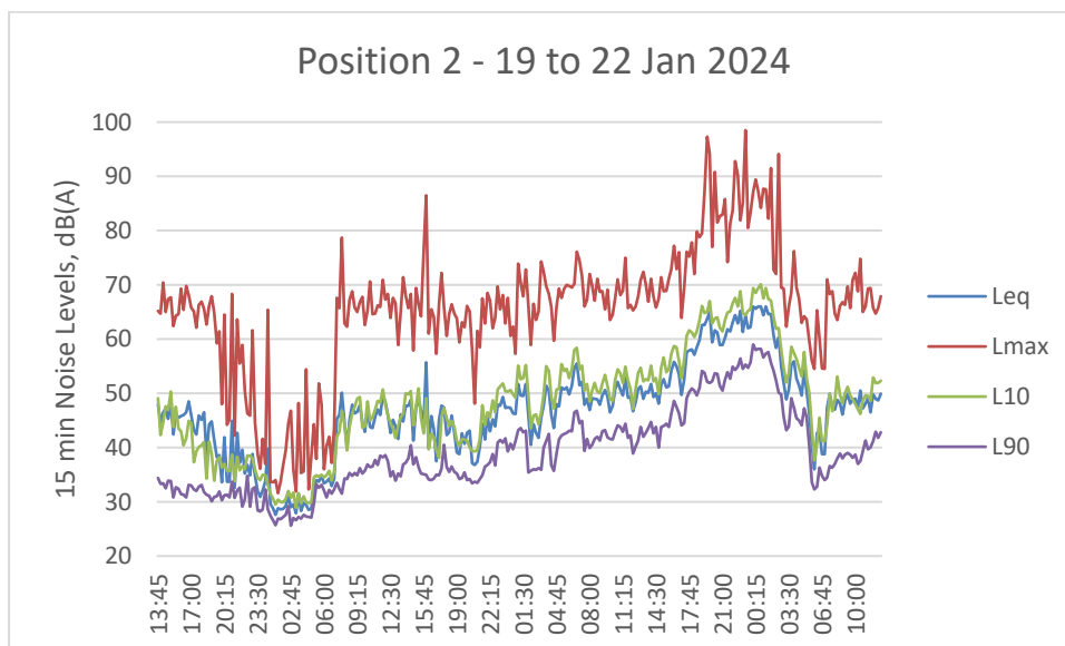
Figure C2: Measured noise levels at Position 2, free-field dB
