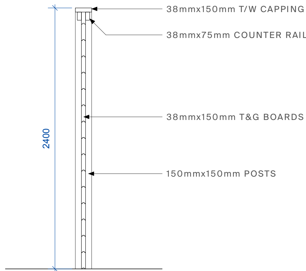
SECTION DETAIL OF ACOUSTIC FENCE 1:20
