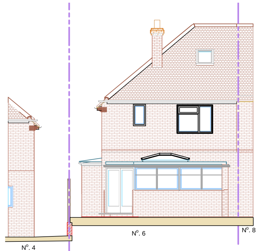
WEST ELEVATION EXISTING SCALE 1:100
