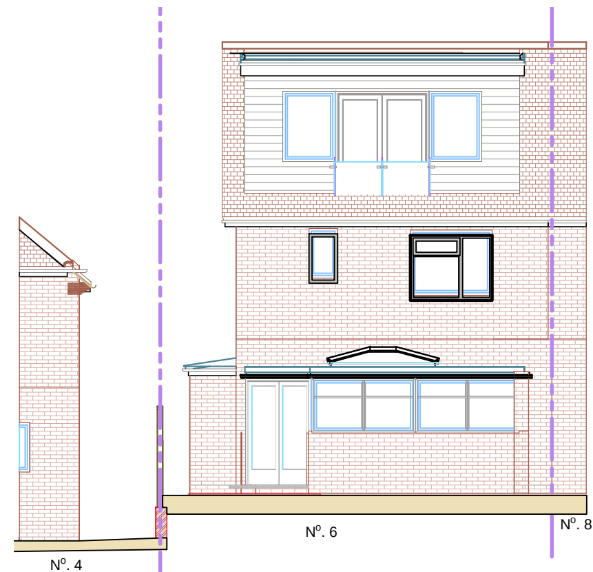
WEST ELEVATION PROPOSED SCALE 1:100
