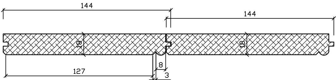
HORIZONTAL DETAIL through BEAD and BUTT WALL BOARDING - Scale 1:2 @ A1
