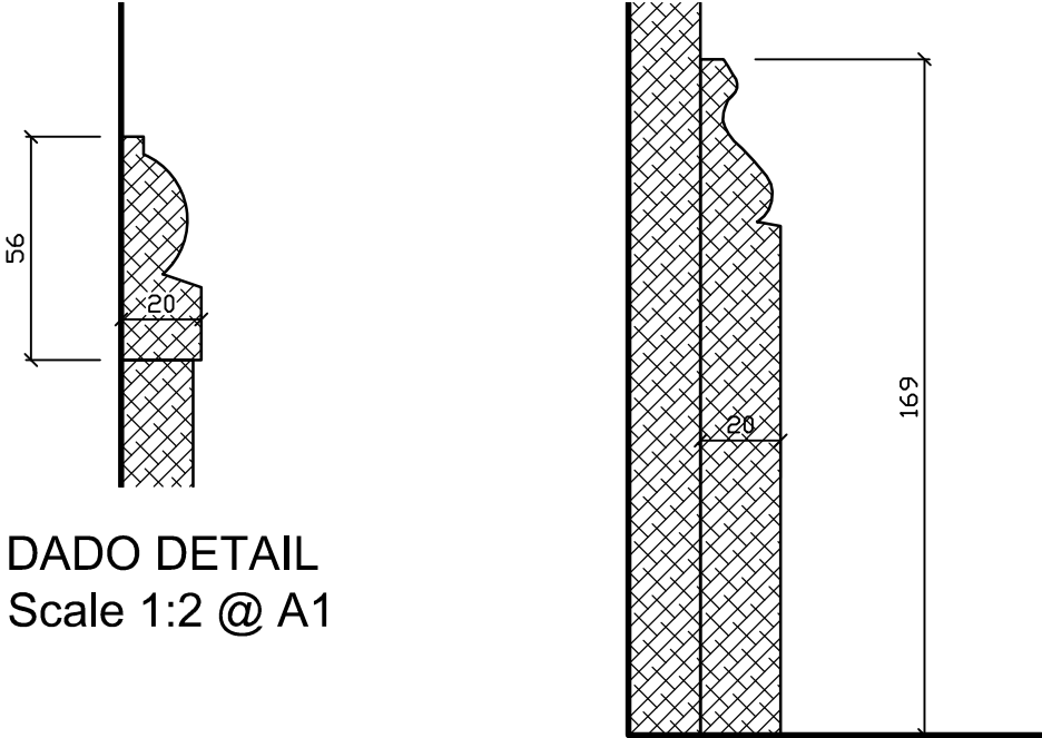
SKIRTING DETAIL Scale 1:2 @ A1
