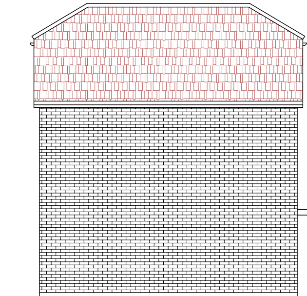
PROPOSED SIDE ELEVATION-02
