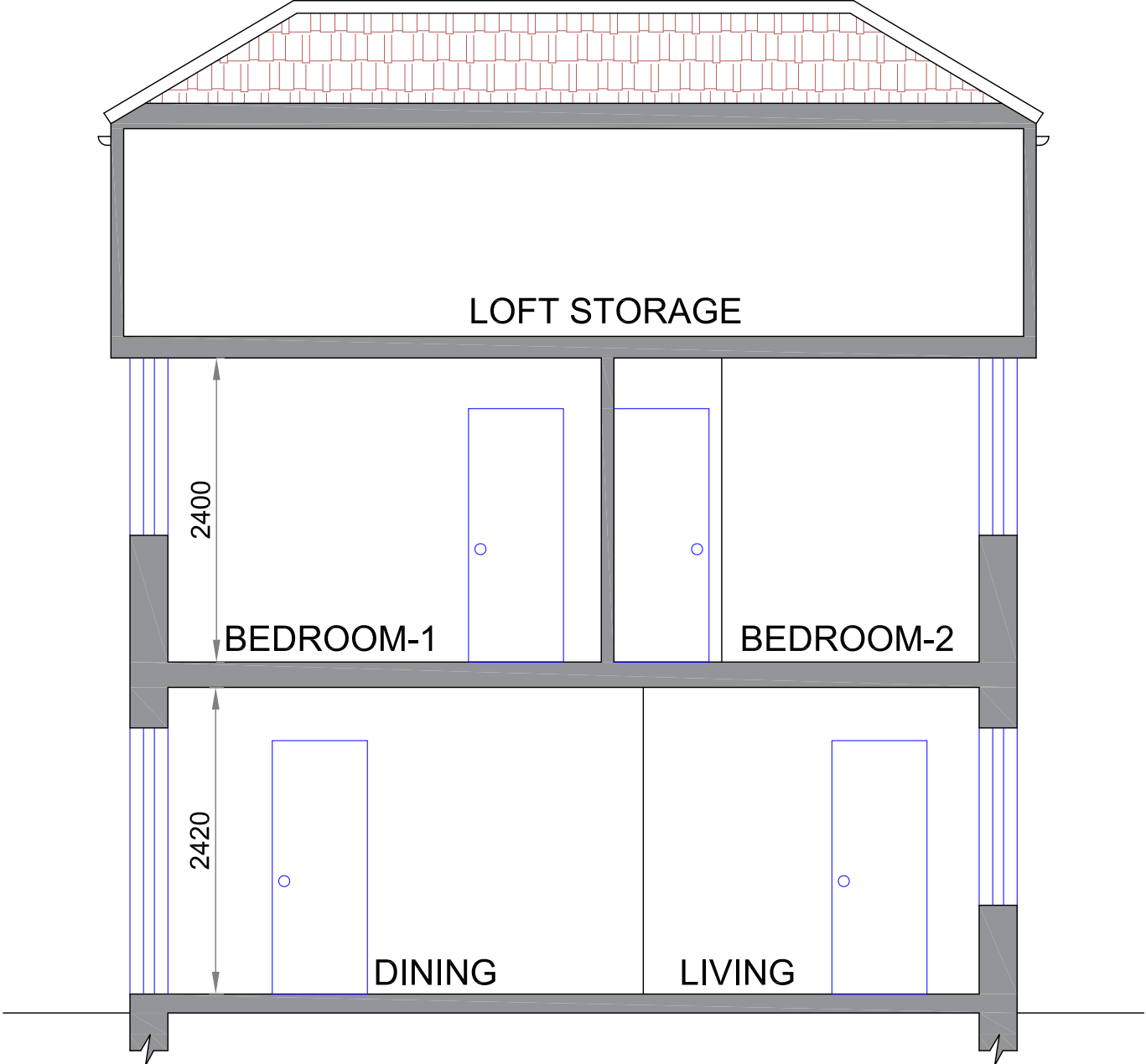
PROPOSED (NEW HOUSE) SECTION AA
