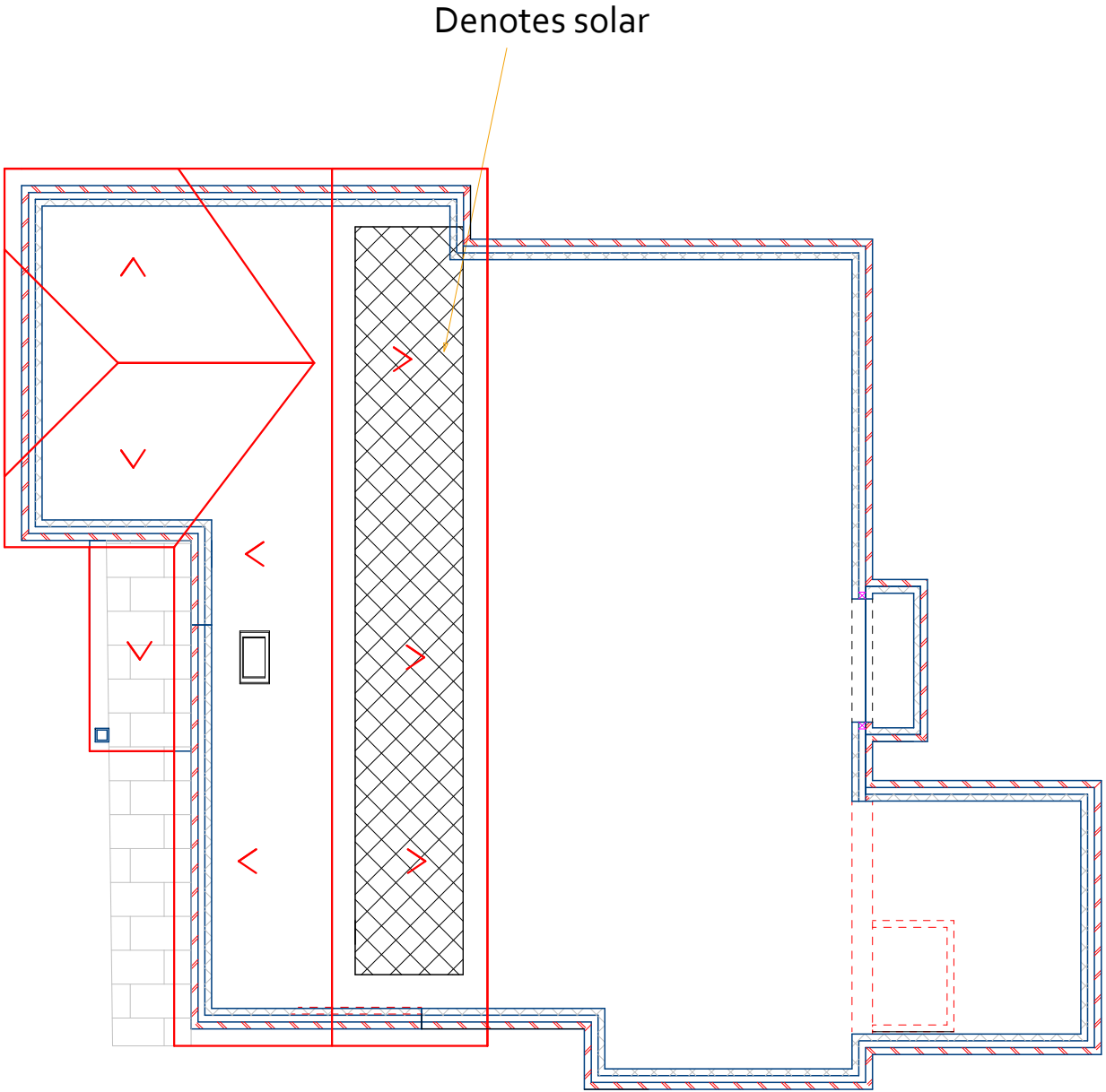
First floor
