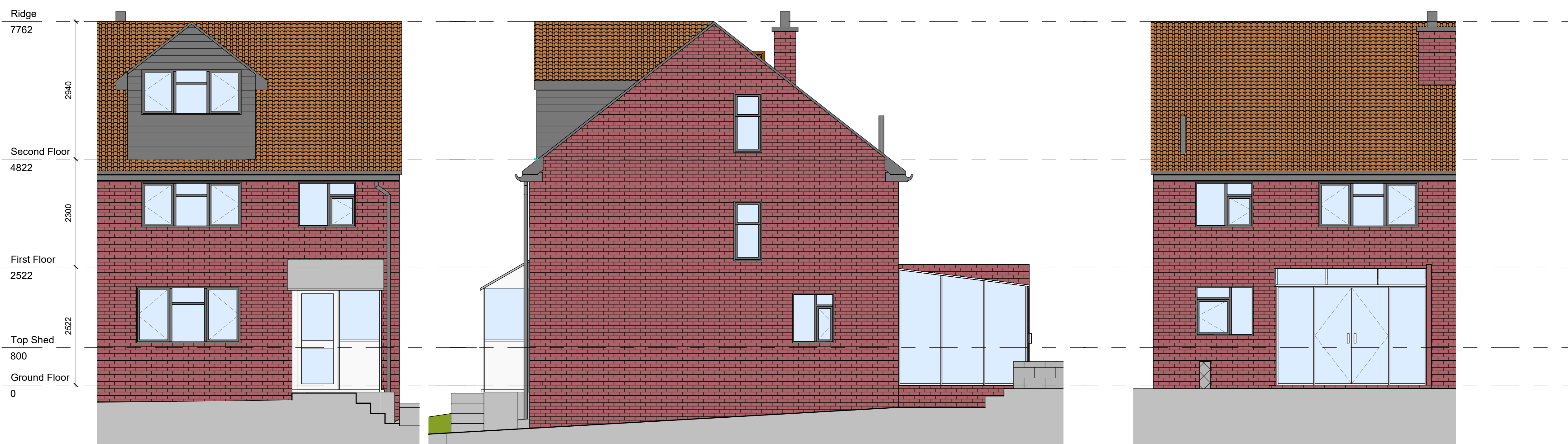
South Existing 01 1 : 50
