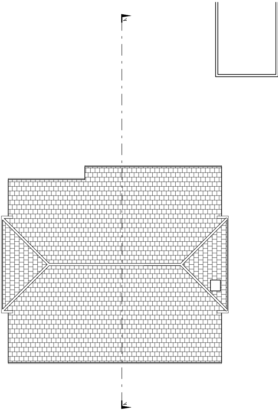
Roof Plan
