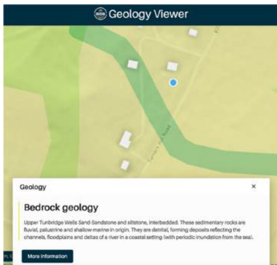
Figure 6 - Bedrock Geology
