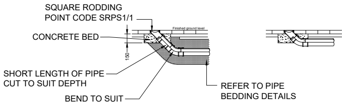
RODDING POINT
