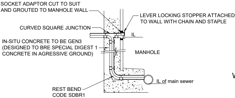
BACK DROP DETAIL FOR CONNECTION TO DEEP MANHOLE
