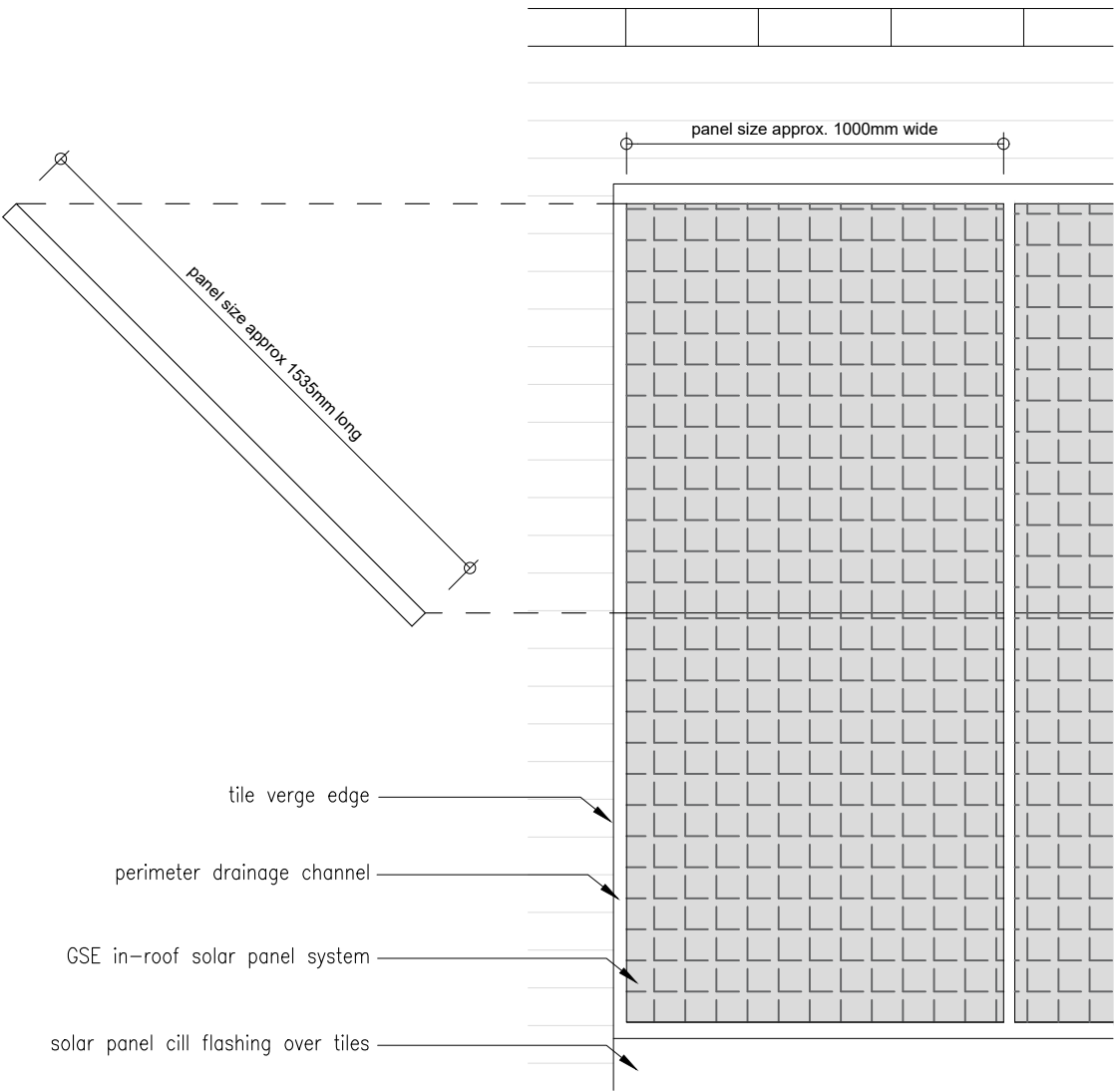
03 PROPOSED CONSTRUCTION BUILD UP - SOLAR PANEL ELEVATION 1:20
