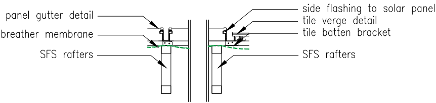
01 PROPOSED CONSTRUCTION BUILD UP - SOLAR PANEL SECTION 1:20
