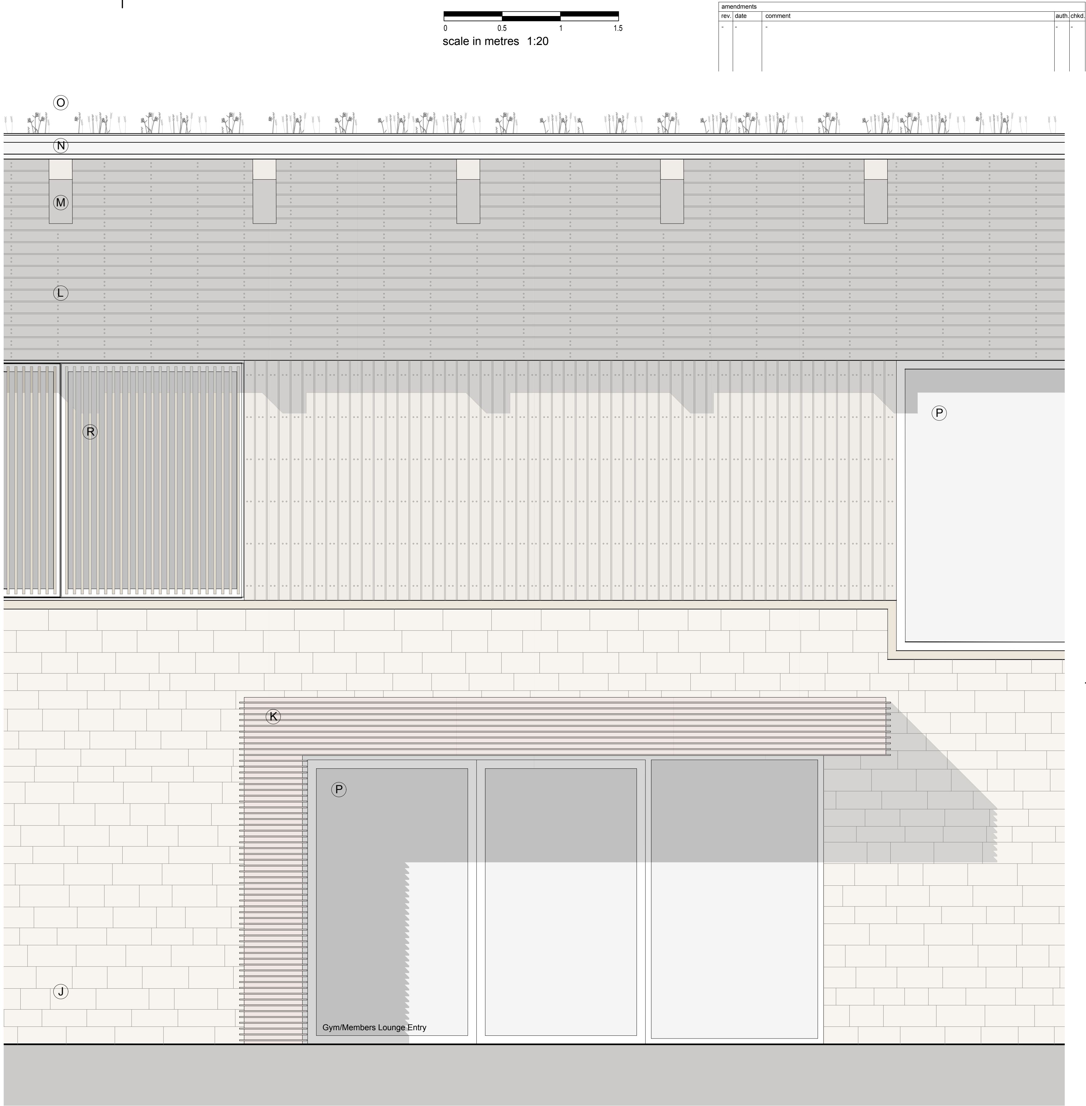
Proposed Detail Elevation 1:20
