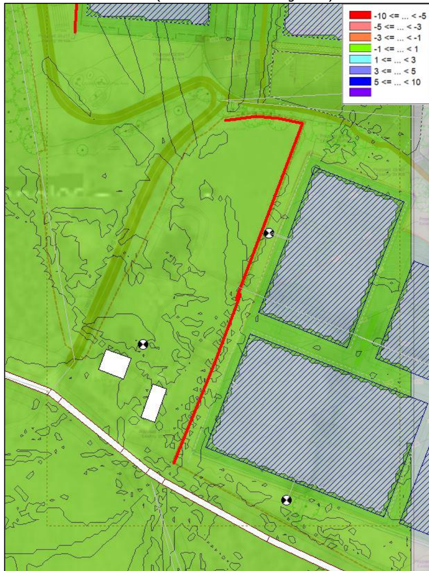
Figure 1: Predicted AGP Noise Emission (1.5 metres above the ground).
