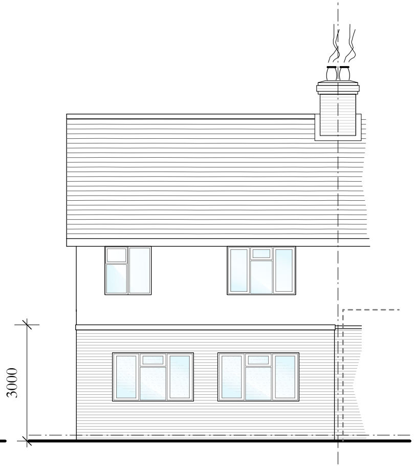
PROPOSED REAR ELEVATION (South East Elevation)
