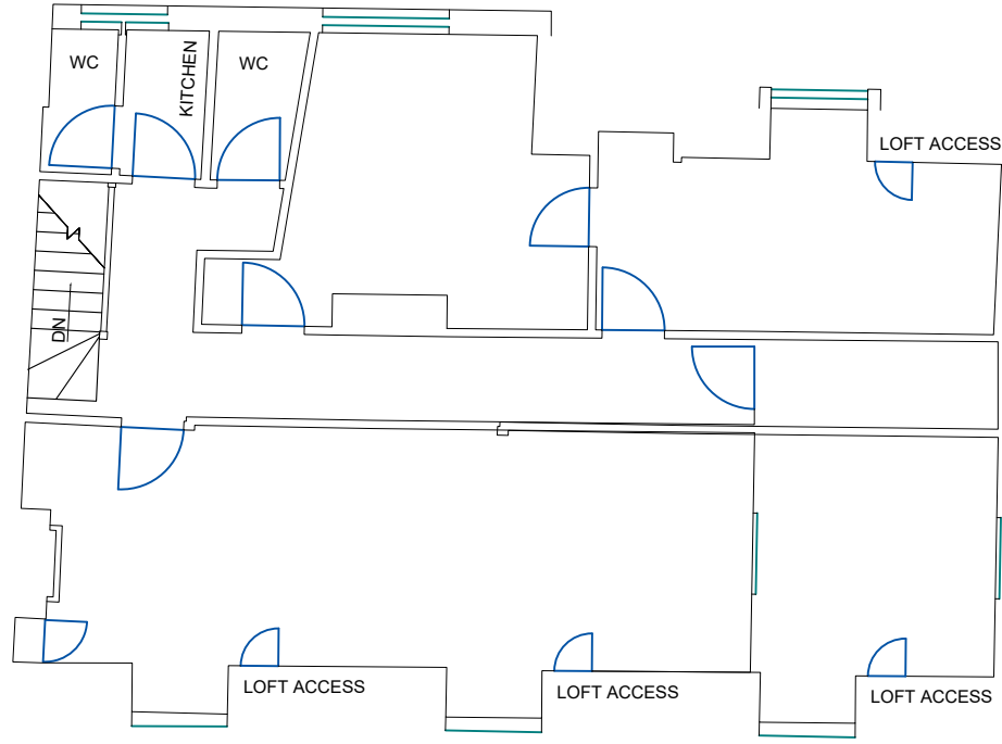
SECOND FLOOR
