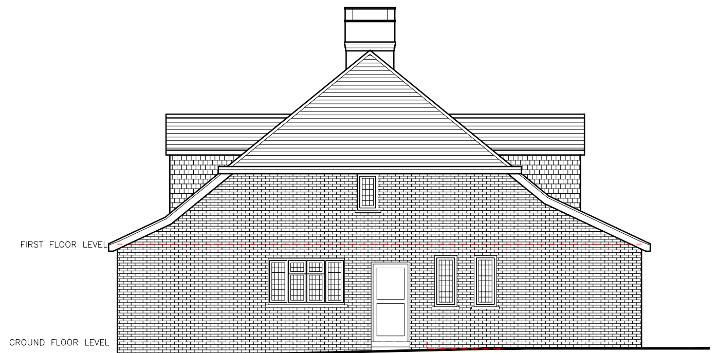
B) Existing Side Elevation
