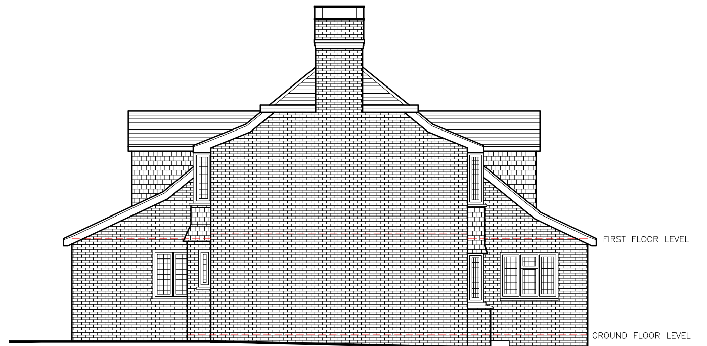
A) Existing Side Elevation
