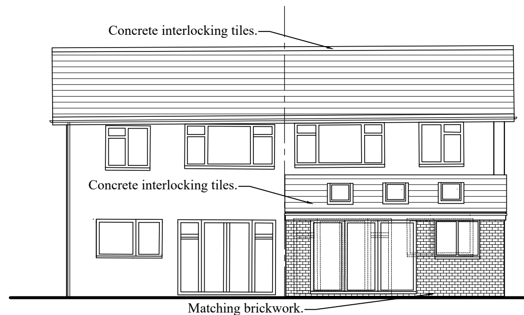
North Elevation
