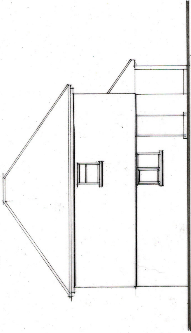
SOUTH ELEVATION
