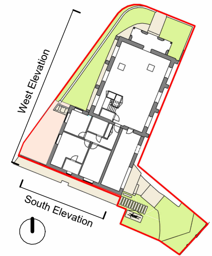
Key plan
